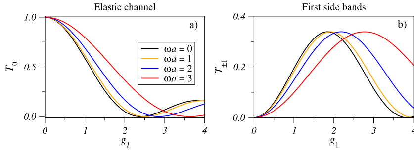
Fig. 1. Transmission probabilities for (a) the central band, T_0 , and (b) the two nearest side bands, T_{\pm 1} , as a function of the bare coupling constant g_1 = V_1 a and different values of the parameter \omega a .
